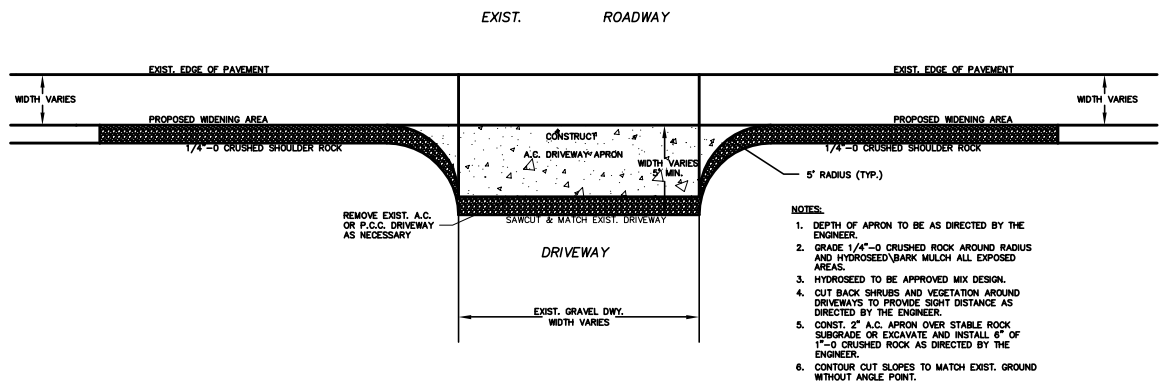
A.C./P.C.C. DRIVEWAY APPROACH CONNECTION N.T.S.
