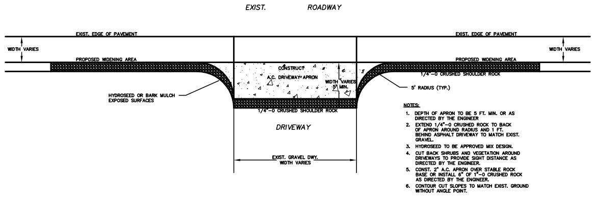
GRAVEL DRIVEWAY APPROACH CONNECTION N.T.S.
