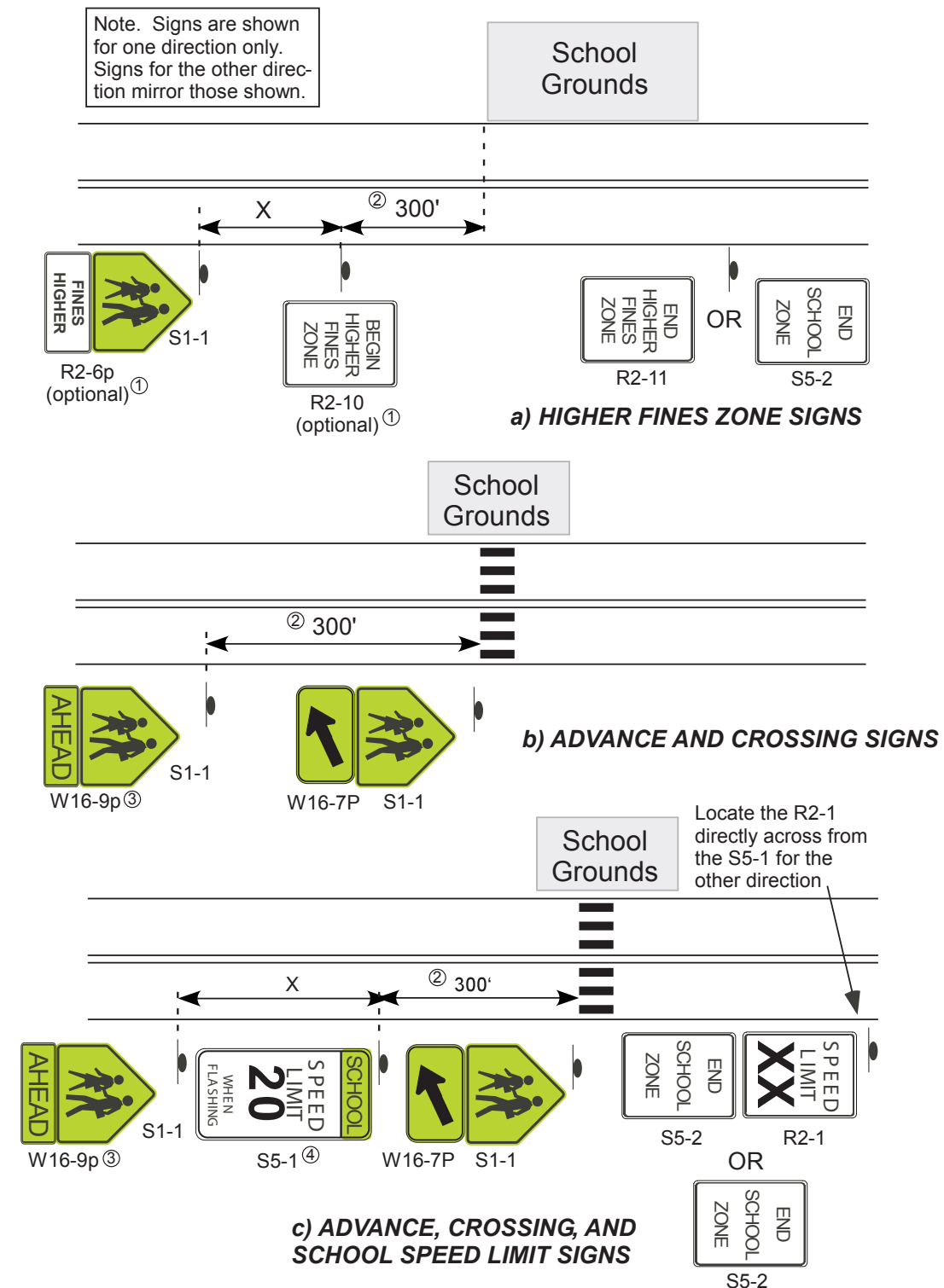
Figure 7B-100. School Zone Traffic Control
