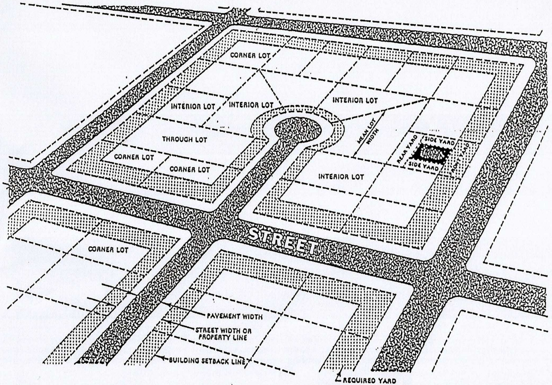
BLOCK DIAGRAM SHOWING LOT TYPES, SET BACKS AND TERMS ...
